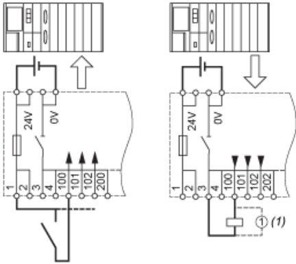
(1) Inductive load
